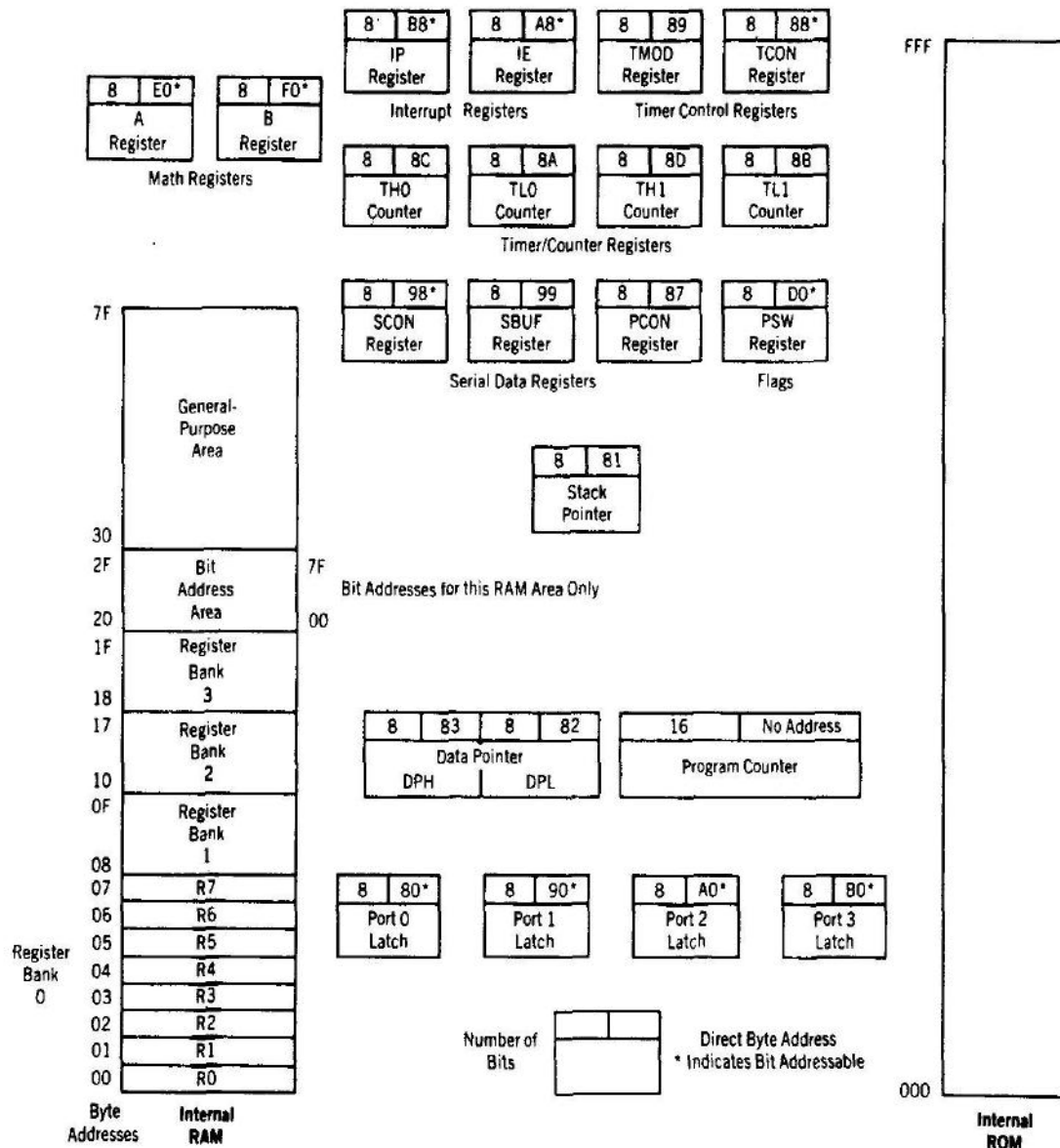
FIGURE 2.1b 8051 Programming Model
