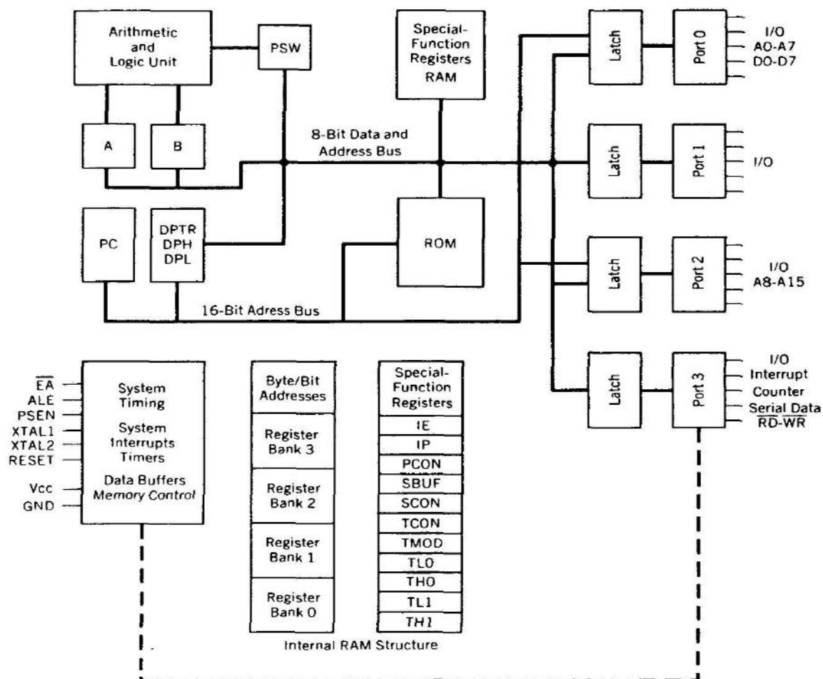
FIGURE 2.1a 8051 Block Diagram
